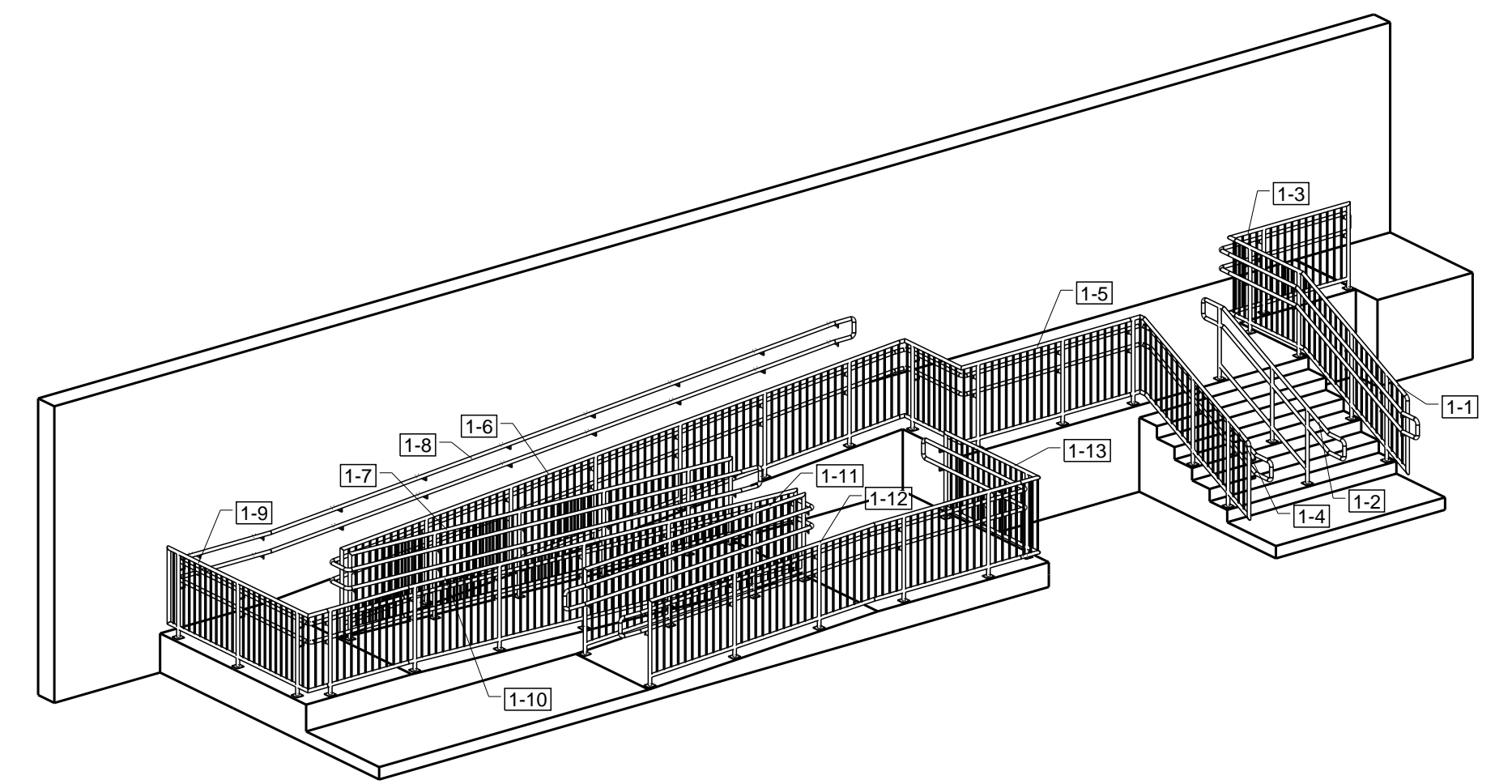
RAMP 3D VIEW
