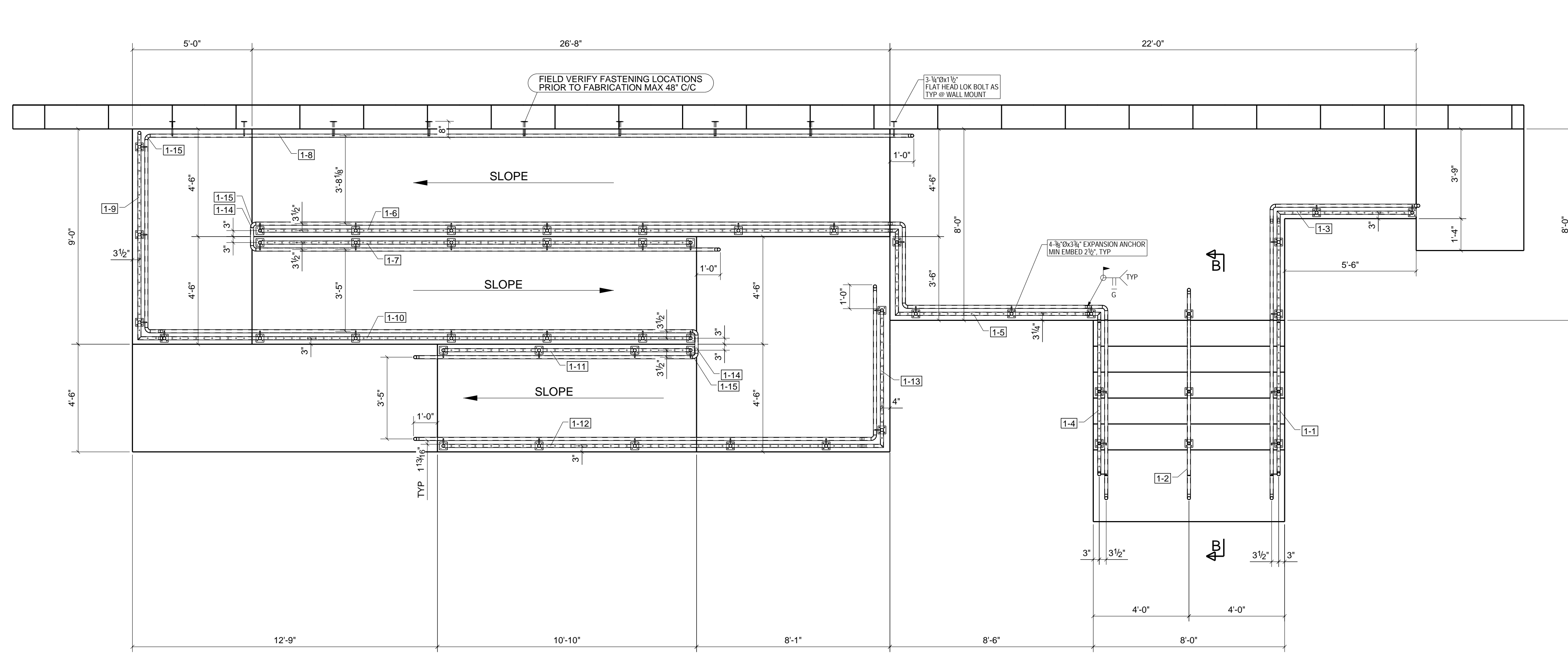
RAMP PLAN VIEW
