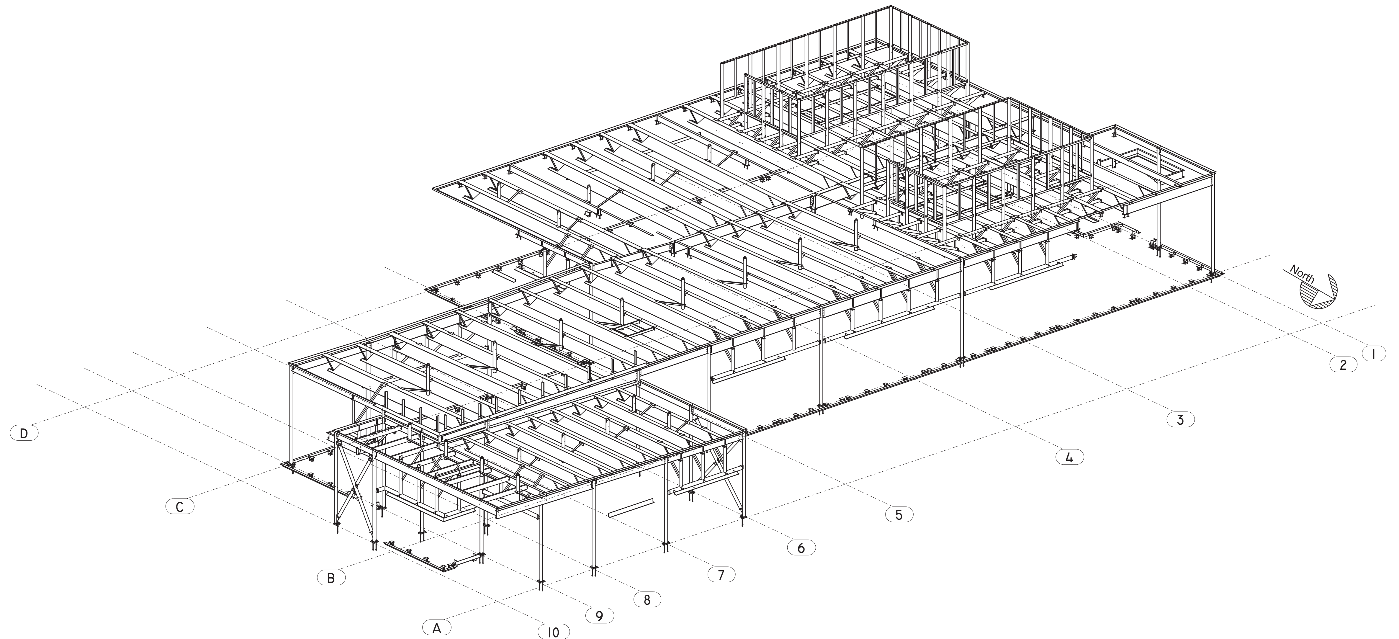
ISOMETRIC VIEW (EAST/WEST)
